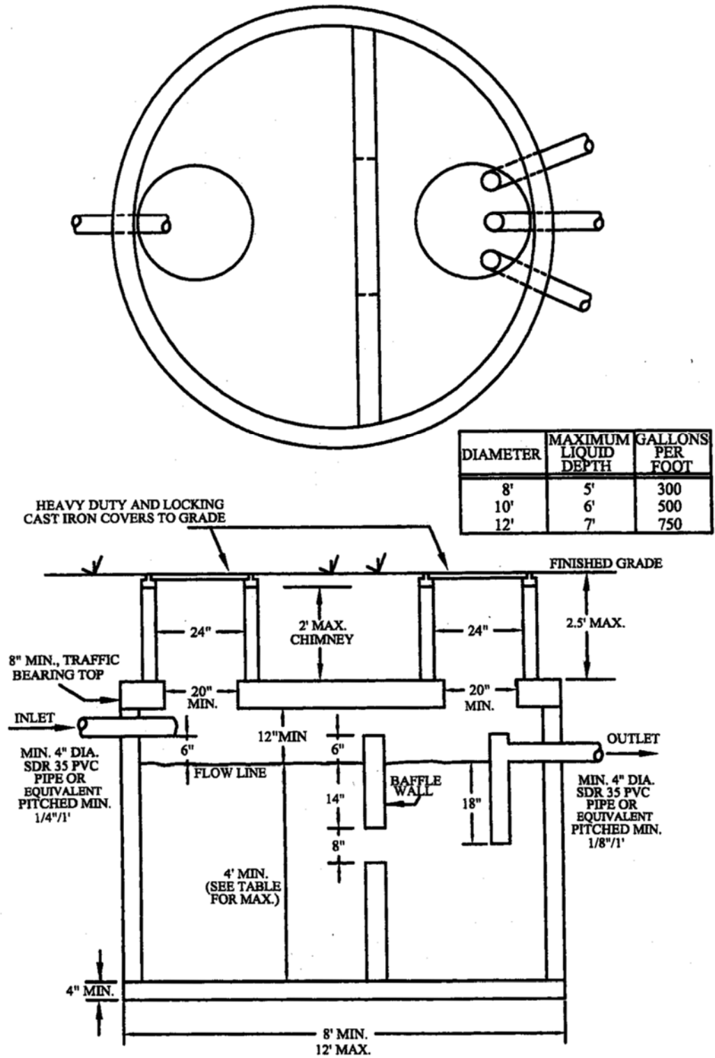
FIGURE 2 SINGLE UNIT CONCRETE SEPTIC TANK
