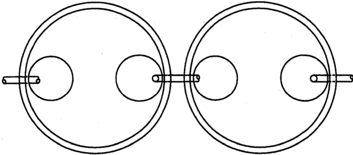
FIGURE 7 MULTIPLE UNIT CONCRETE GREASE TRAP (2 Tank Example)
